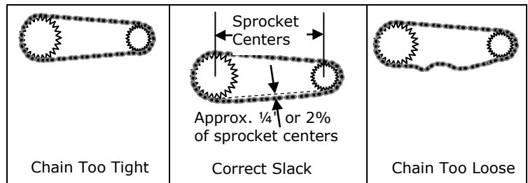
Figure 5.2 Drive Chain Sag
